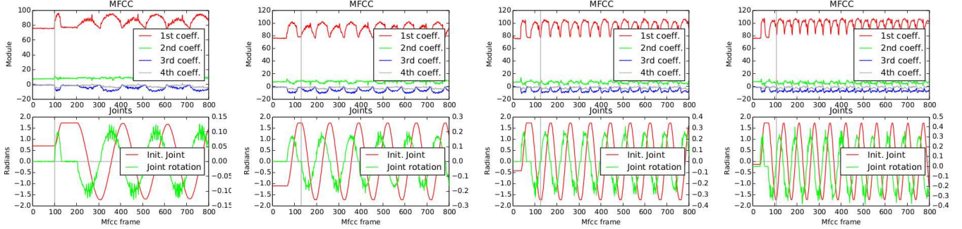
Figure 4: Example of trajectories of synchronised audio-motor data from the four velocity profiles. The upper plot shows the trajectories of the first 4-MFCC coefficients extracted from the single channel auditory signal recorded while executing the head rotations. The plot in the bottom shows the head yaw joint position (red line) and the head yaw rotation over 40ms (green line). The columns represent the different velocity profiles. From left to right: slow , medium , fast and very fast .
